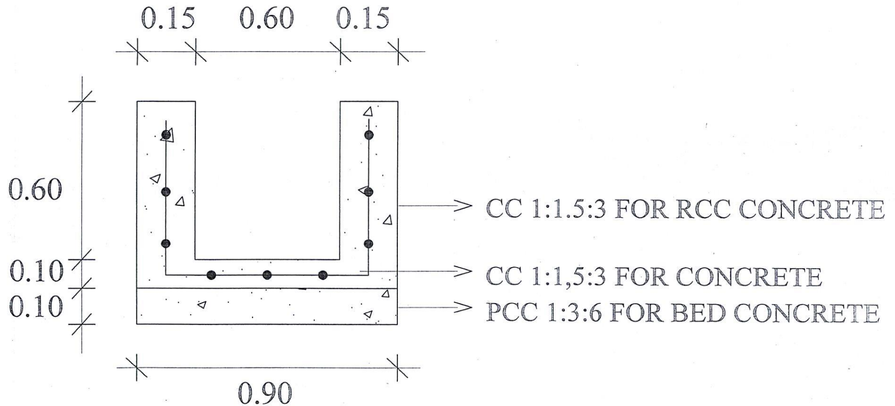
C / SECTION OF DRAINAGE
